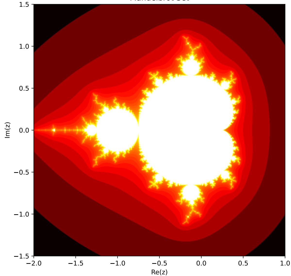
Mandelbrot Set
